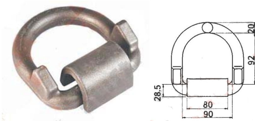
D-ring With Supporting Point
